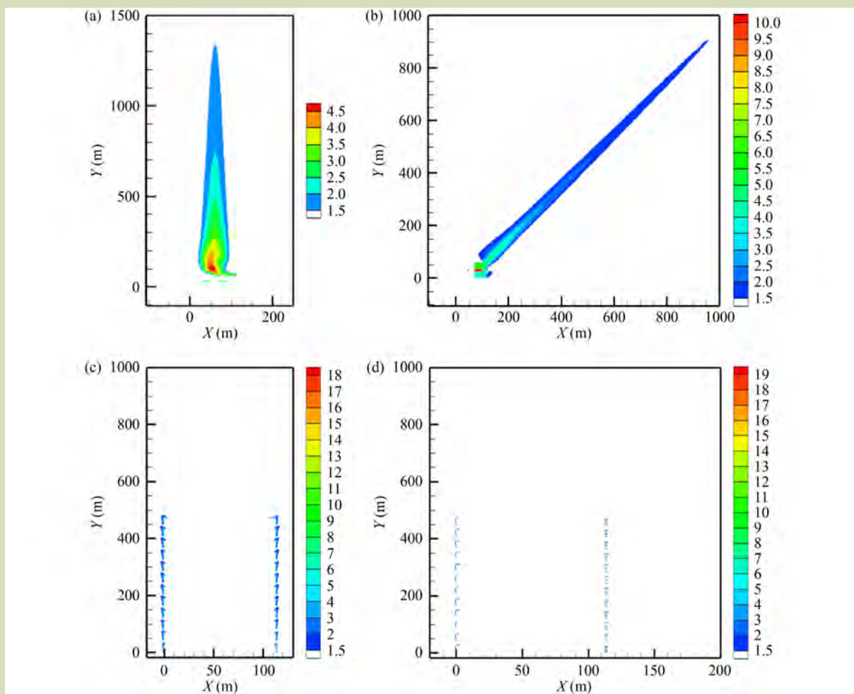
Fig. 14 Ammonia concentration gradient (ppmv) on the plane Z = 1.5 m under different wind directions, wind speed of 2 \text{ m}\cdot\text{s}^{-1} and emission source concentration of 20 ppmv: (a) 90^\circ , the multi-floor pig building; (b) 135^\circ , the multi-floor pig building; (c) 90^\circ , the flat-floor pig farm; (d) 135^\circ , the flat-floor pig farm.
