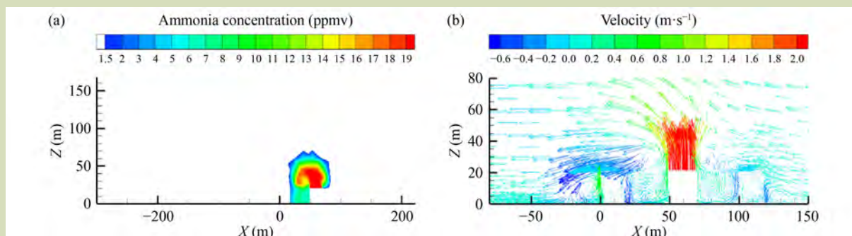
Fig. 13 Plane Y = 31 m of the multi-floor pig building: (a) ammonia concentration distribution; (b) velocity vector distribution.
